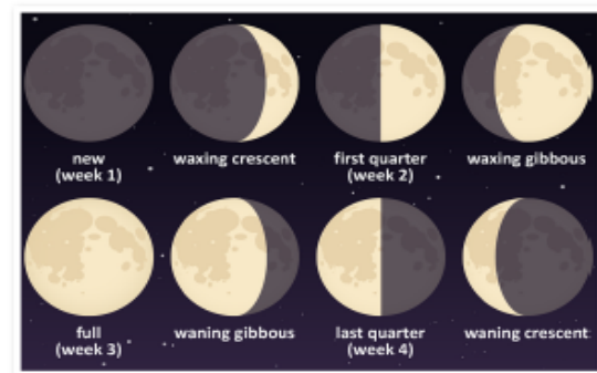
Phases of the Moon
